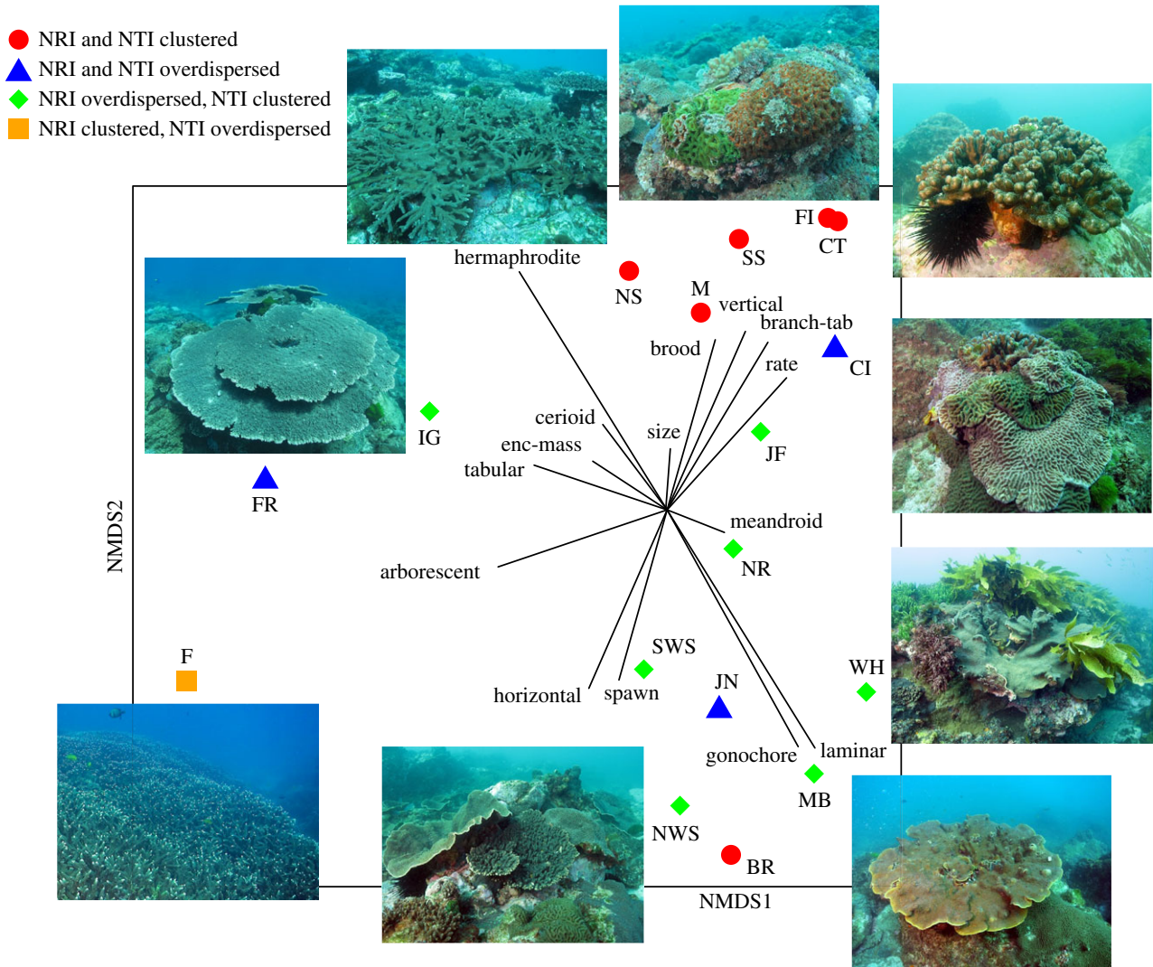
Figure 3. Non-parametric multidimensional scaling ordination of phylogenetic diversity patterns of corals on high-latitude reefs in eastern Australia. The ordination is based on the abundance-weighted net relatedness index (NRI ab ) and symbols represent patterns in phylogenetic structure at the study sites as indicated in the legend; see figure 2 for abbreviations of site names. Vectors identify traits that primarily discriminate assemblages: enc-mass, encrusting-to-massive morphology; branch-tab, branching-to-tabular morphology; rate, larval development rate; size, corallite size. Photos portray assemblage types at the study sites. All photos by B. Sommer.
